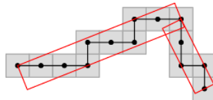
Figure 2: Example of a 4-DSS decomposition of a small point sequence.
