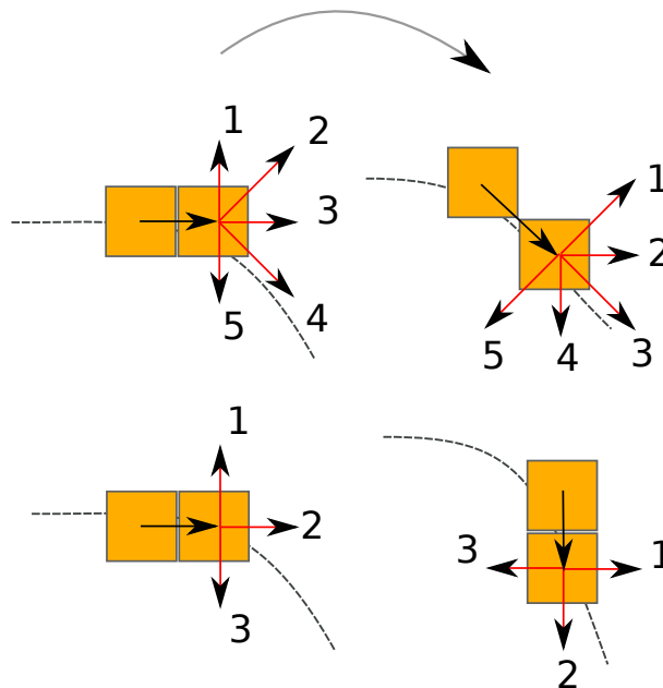
Figure 1: Illustration of the border tracker algorithm.
